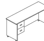
COS-202 (1200×420×670)
